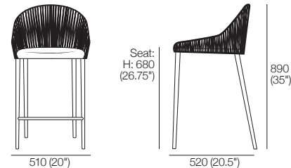
Counter Stool (Woven) Front View | Side View
